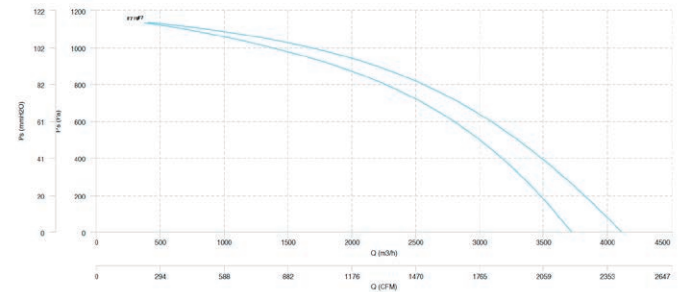
DOMEX 3900 EEC H DOMEX 3900 EEC V
