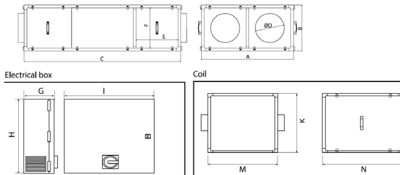
Dimensions DOMEX EEC Series (Horizontal installation)
