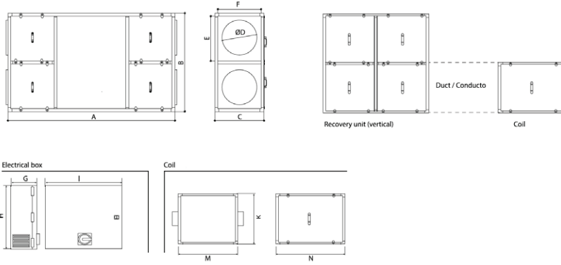
Dimensions DOMEX EEC Series (Vertical installation)
