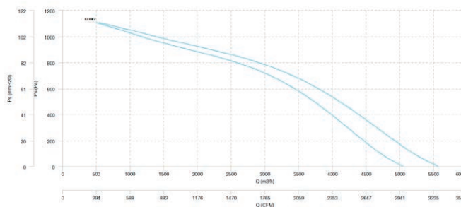
DOMEX 5400 EEC H DOMEX 5400 EEC V
