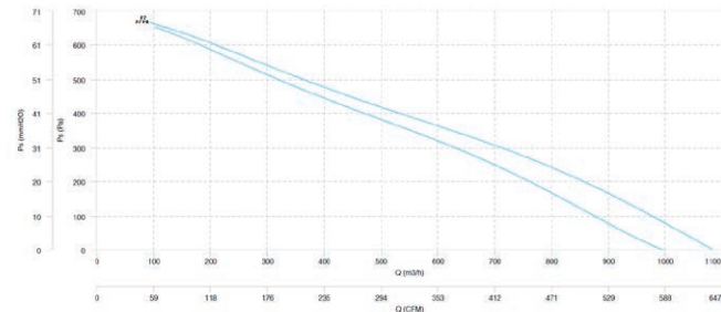
DOMEX 2300 EEC H DOMEX 2300 EEC V
