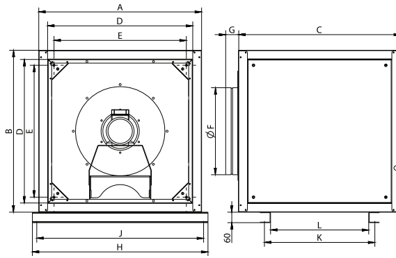
Dimensions BOX RLF Series
