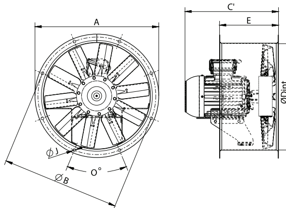
Dimensions Series HC / HCA 230 V (mm)
