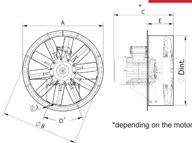
Dimensions HB / HBA Series 230V
