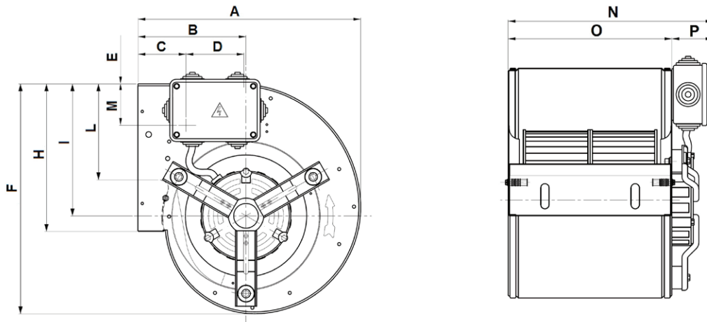
Dimensions DD Series 900 RPM 3 Speed (mm)
