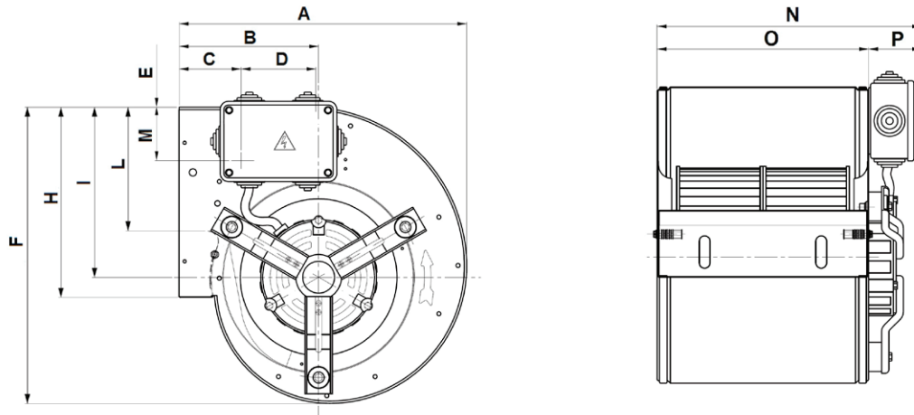
Dimensions DD Series 900 RPM 1 Speed
